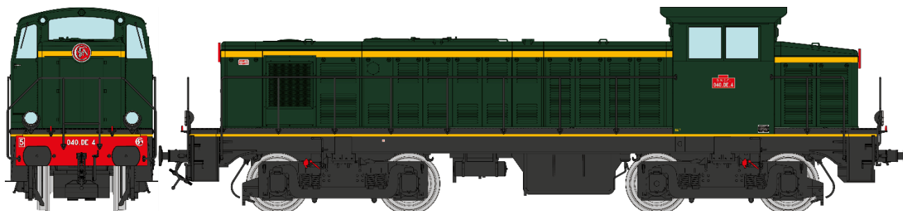
040 DE 4, Livrée d'origine, plaques en relief, Ep. III Diesel Locomotive 040 DE 4, Origin livery, raised road number plates, SNCF Period III
